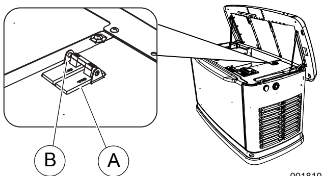
Figura 3-3. Disyuntor principal
