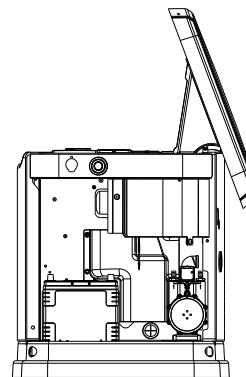
RIGHT VIEW INTAKE PANEL REMOVED
