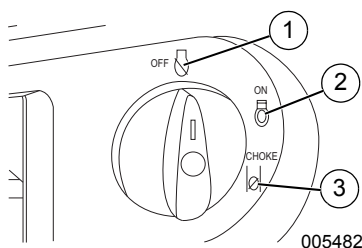
Figure 2-5. Switch (example)
