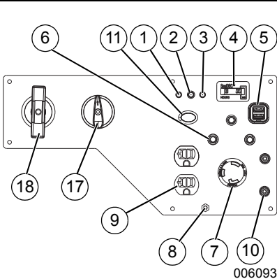
Figure 2-2. Control Panel
