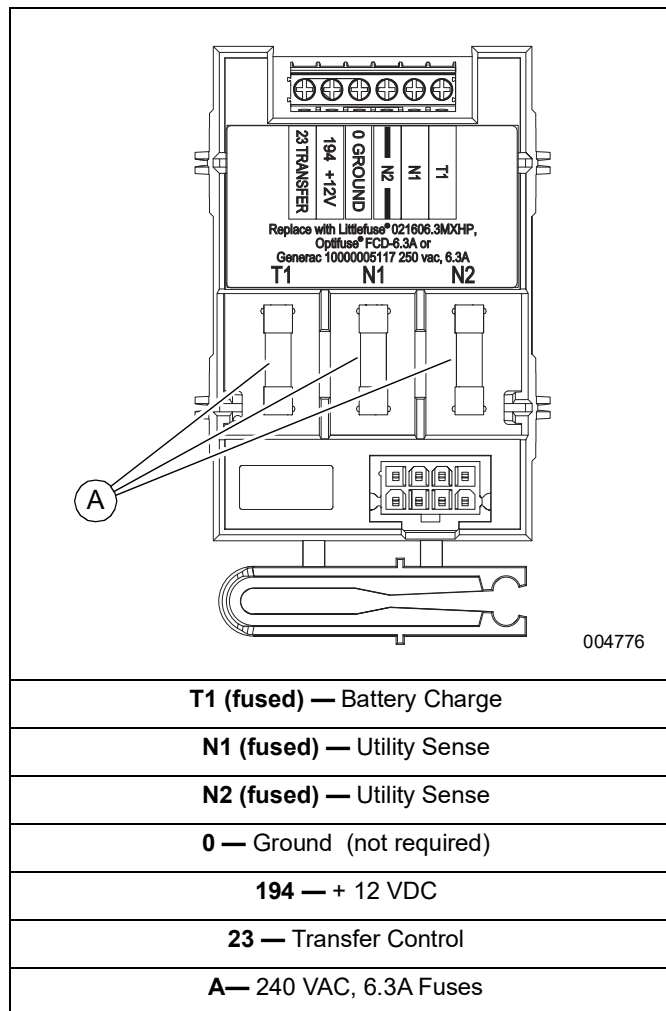
Figure 3-2. Typical Connections
