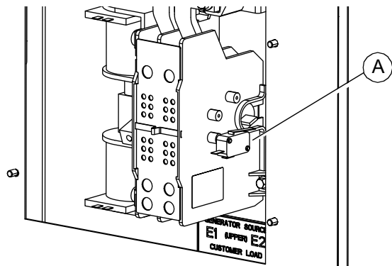
Figure 3-3. Auxiliary Contact
