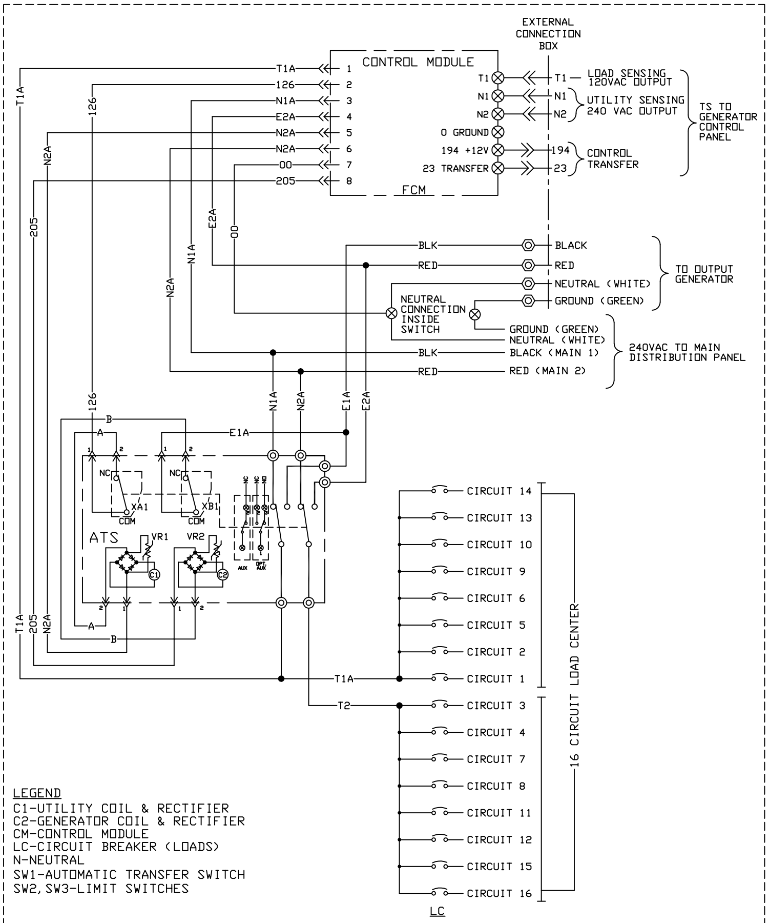
SCHEMATIC - DIAGRAM HSB TRANSFER SWITCH 100A DRAWING #:10000018987
