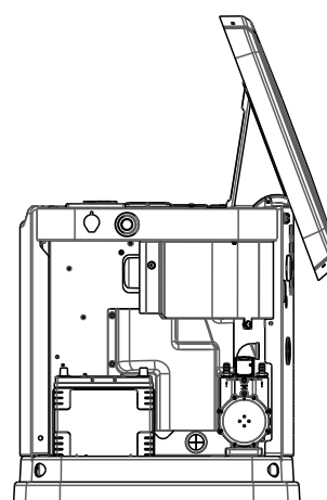
RIGHT VIEW INTAKE PANEL REMOVED
