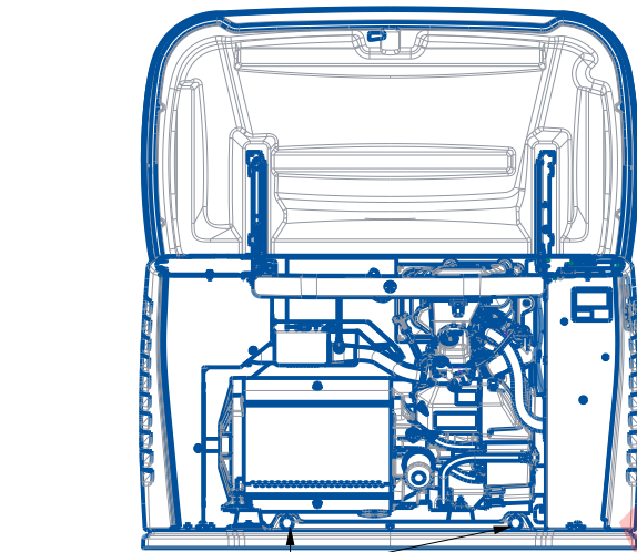
FRONT VIEW FRONT PANEL REMOVED ROOF OPENED
