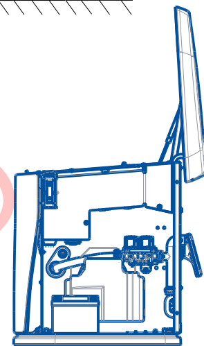
RIGHT SIDE VIEW INTAKE PANEL REMOVED
