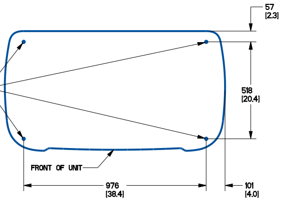
MOUNTING TO CONCRETE PAD
