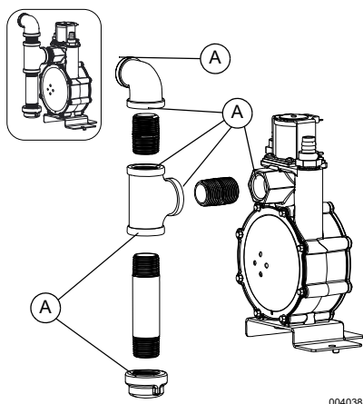
Figure 4-12. Vérification des fuites aux points de raccordement
