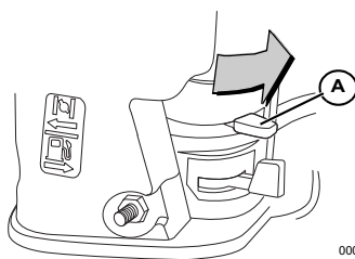
Figure 3-6. Fuel Valve and Choke
