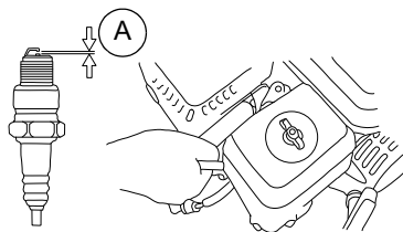
Figure 4-13. Spark Plug
