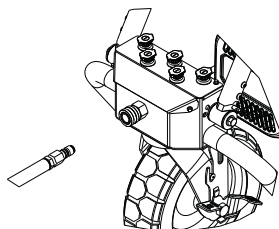
Figure 2-9. Connect High-Pressure Hose to Quick Connect Fitting
