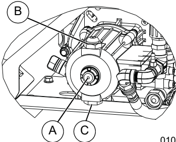
Figure 4-6. Drain/Fill Oil
