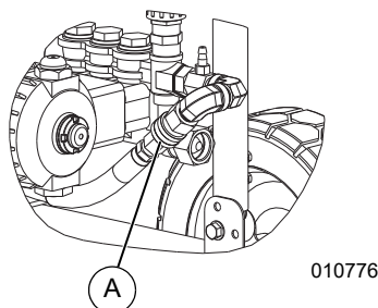
Figure 4-15. Disconnect Pump Hose
