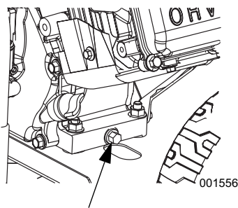
Figure 4-12. Oil Drain Plug
