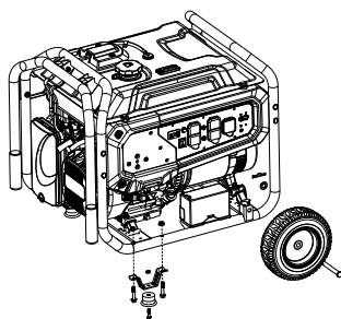
Figure 2-8. Wheel & Foot Assembly
