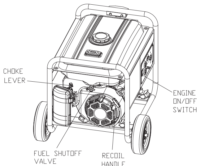
Figure 11 - Engine Controls
