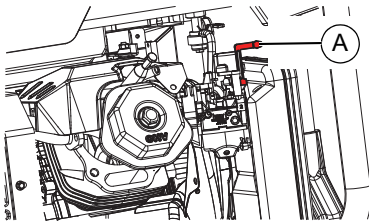
Figure 3-4. Choke Lever
