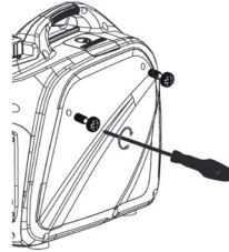
Figure 2-6. Remove Side Cover
