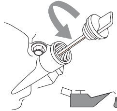
Figure 2-7. Remove Dipstick
